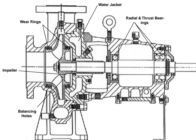
Figure 1 - Typical high pressure, high temperature process pump
